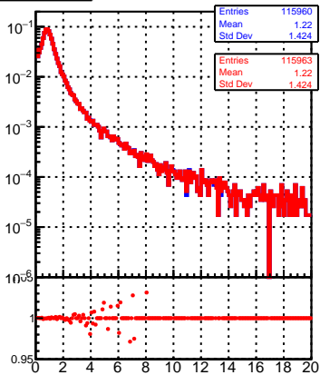
normalized \chi^2
