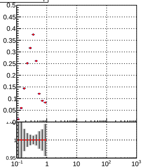
■ DQM_TT_mkFit-DQM_pless_orig ◆ DQM_TT_mkFit-DQM_pless_modi2
