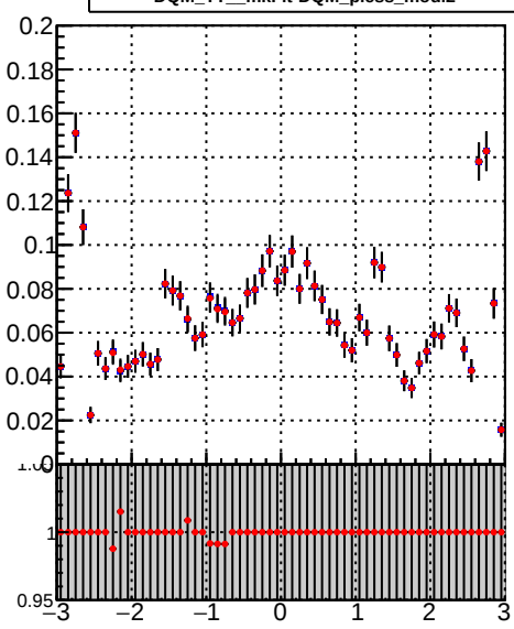
— DQM_TT_mkFit-DQM_pless_orig — DQM_TT_mkFit-DQM_pless_modi2
