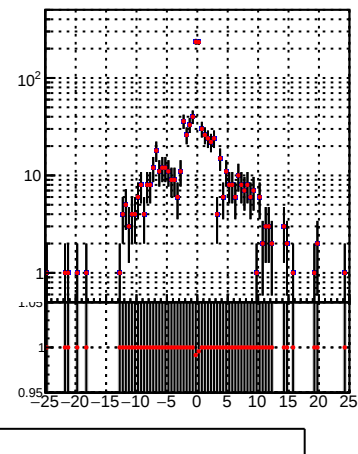
N of associated tracks (simToReco) vs dxy(PV)
