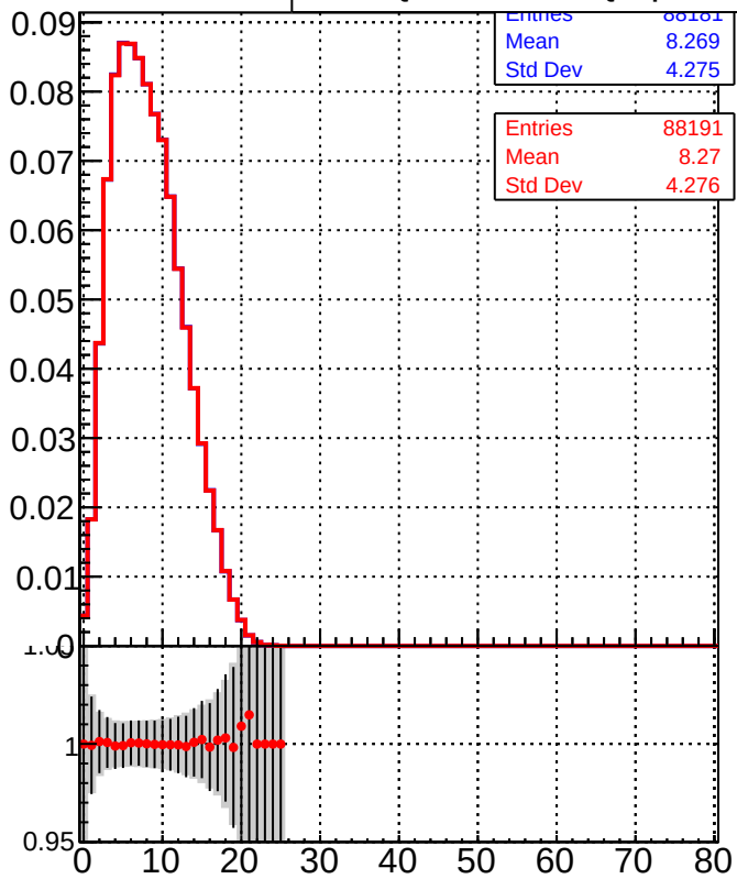
Legend: DQM_TT_mkFit-DQM_pless_orig (grey histogram) DQM_TT_mkFit-DQM_pless_modi2 (red line with markers)
