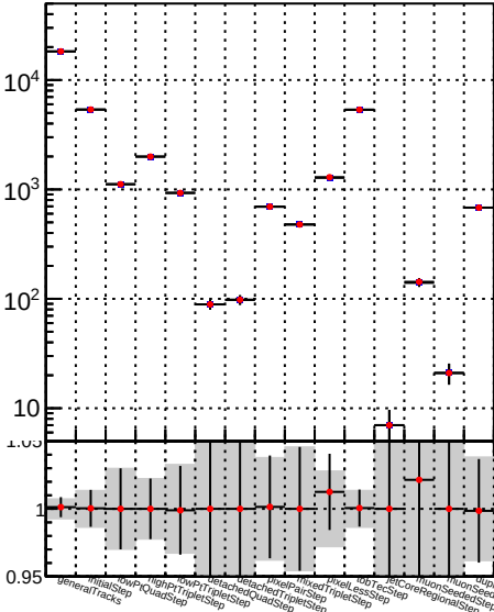
Number —●— DQM_TT__mkFit-DQM_pless_mod
