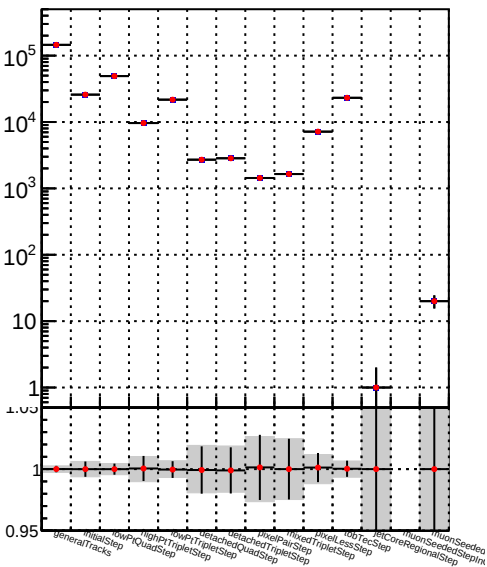
Number —●— DQM_TT__mkFit-DQM_pless_mod
