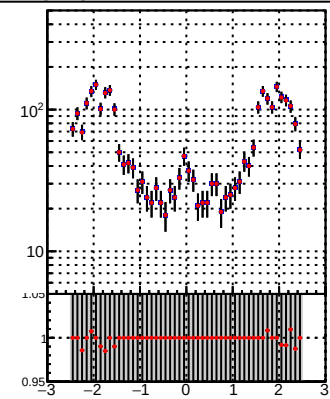
—●— DQM_TT_mkFit-DQM_pless_orig —●— DQM_TT_mkFit-DQM_pless_modi2
