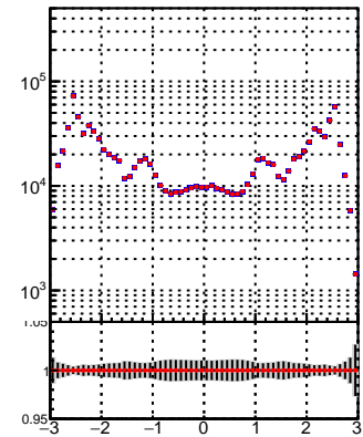
N of reco track vs \eta DQM_TT_mkFit-DQM_pless_orig N of reco track vs \eta DQM_TT_mkFit-DQM_pless_modi2
