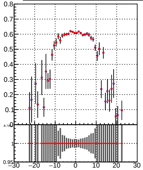
Efficiency vs. sim PV z — DQM_TT_mkFit-DQM_pless_orig — DQM_TT_mkFit-DQM_pless_modi2
