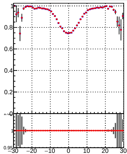
—•— DQM_TT_mkFit-DQM_pless_orig —•— DQM_TT_mkFit-DQM_pless_modi2
