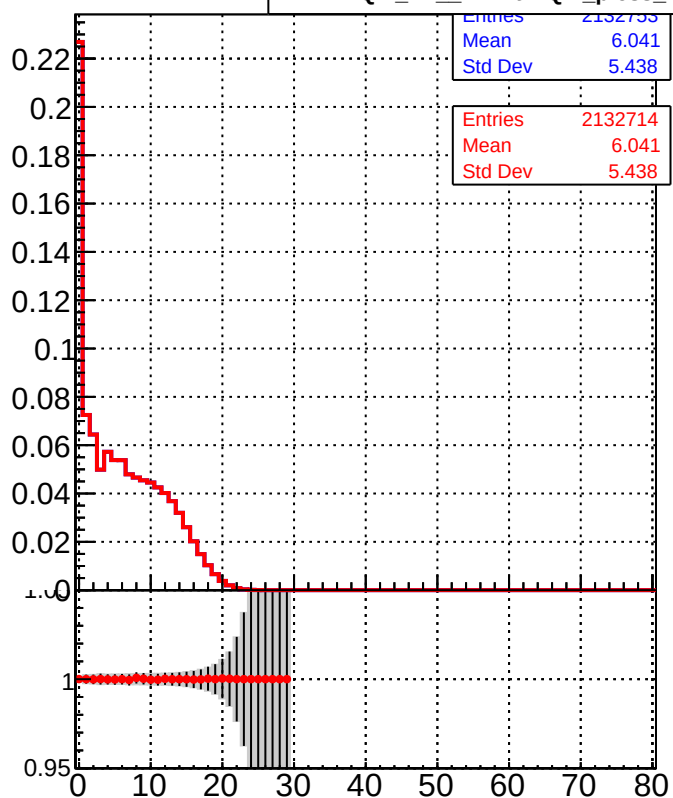
— DQM_TT_mkFit-DQM_pless_orig — DQM_TT_mkFit-DQM_pless_modi2
