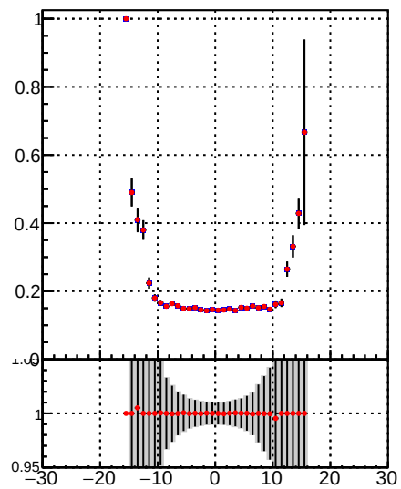
Fake rate vs d —●— DQM TT mkFit-DQM_pless_orig —●— DQM TT mkFit-DQM_pless_modi2
