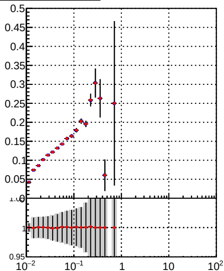
—•— DQM_TT_mkFit-DQM_pless_orig —•— DQM_TT_mkFit-DQM_pless_modi2
