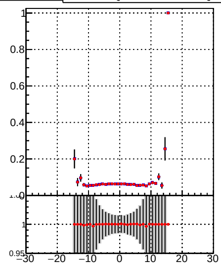
—•— DQM_TT_mkFit-DQM_pless_orig —•— DQM_TT_mkFit-DQM_pless_modi2
