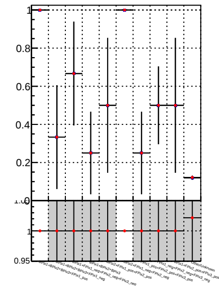
Fake rate vs. —•— DQM_TT_mkFit-DQM_pless_orig —•— DQM_TT_mkFit-DQM_pless_modi2
