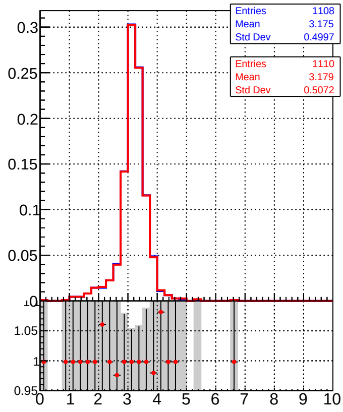
Legend: DQM_TT_mkFit-DQM_pless_orig (blue line with squares) DQM_TT_mkFit-DQM_pless_modi2 (red line with circles)
