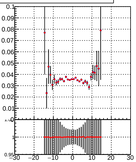
— DQM_TT_mkFit-DQM_pless_orig — DQM_TT_mkFit-DQM_pless_modi2
