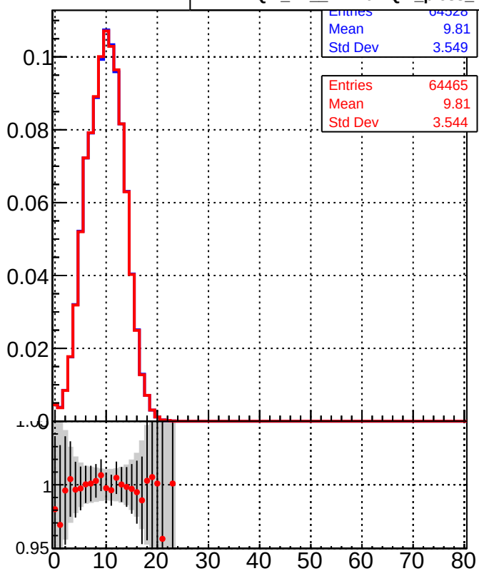
Legend: DQM_TT_mkFit-DQM_pless_orig DQM_TT_mkFit-DQM_pless_modi2
