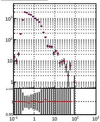
—•— DQM_TT_mkFit-DQM_pless_orig —•— DQM_TT_mkFit-DQM_pless_modi2
