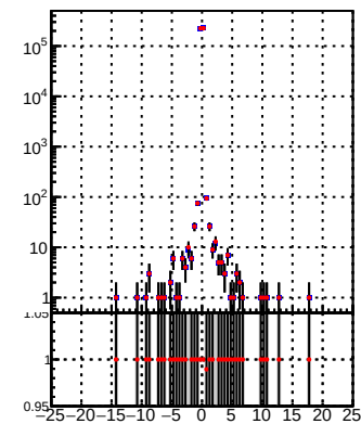
Legend: DQM_TT_mkFit-DQM_pless_orig (black histogram) DQM_TT_mkFit-DQM_pless_modi2 (red dashed line)
