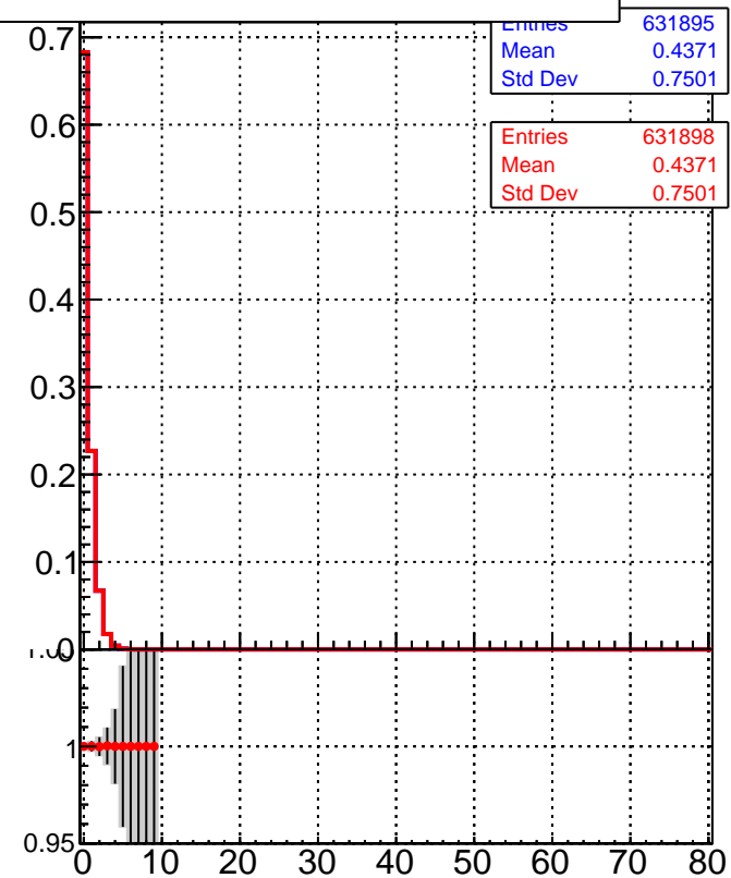
Legend: DQM_TT_mkFit-DQM_pless_orig (grey histogram), DQM_TT_mkFit-DQM_pless_modi2 (red line)
