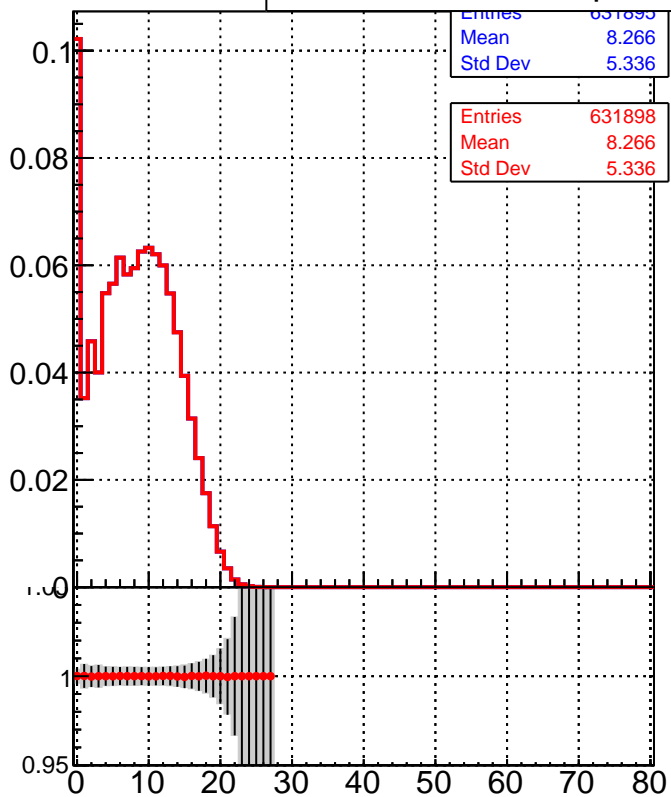
Legend: DQM_TT_mkFit-DQM_pless_orig (grey histogram), DQM_TT_mkFit-DQM_pless_modi2 (red line)
