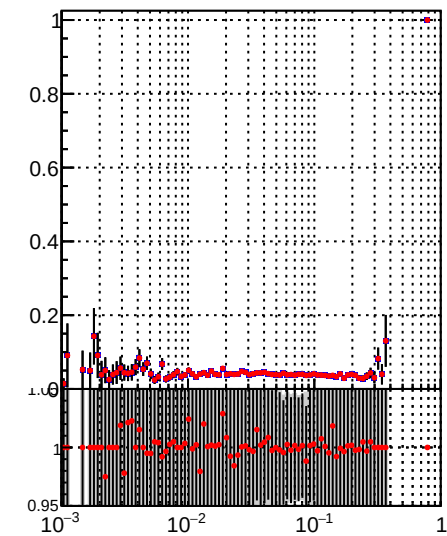
—•— DQM_TT_mkFit-DQM_pless_orig —•— DQM_TT_mkFit-DQM_pless_modi2
