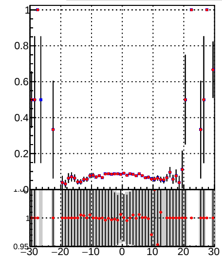
—■ DQM_TT_mkFit-DQM_pless_orig —● DQM_TT_mkFit-DQM_pless_modi2
