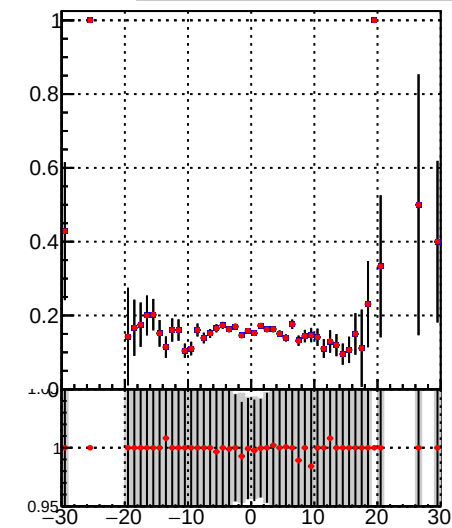
—•— DQM_TT_mkFit-DQM_pless_orig —•— DQM_TT_mkFit-DQM_pless_modi2
