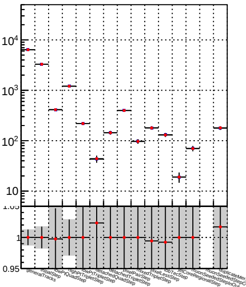
Number —●— DOM TT mkFit-DOM pless mod2
