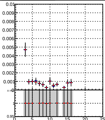
DQM_TT_mkFit-DQM_pless_orig
