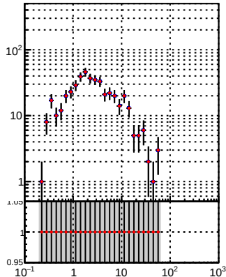
—•— DQM_TT_mkFit-DQM_pless_orig —•— DQM_TT_mkFit-DQM_pless_modi2
