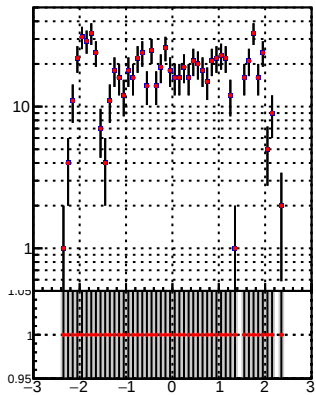
—•— DQM_TT_mkFit-DQM_pless_orig —•— DQM_TT_mkFit-DQM_pless_modi2
