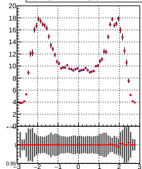
— DQM_TT_mkFit-DQM_pless_orig — DQM_TT_mkFit-DQM_pless_modi2
