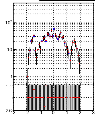
—•— DQM_TT_mkFit-DQM_pless_orig —•— DQM_TT_mkFit-DQM_pless_modi2
