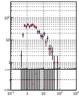
—•— DQM_TT_mkFit-DQM_pless_orig —•— DQM_TT_mkFit-DQM_pless_modi2
