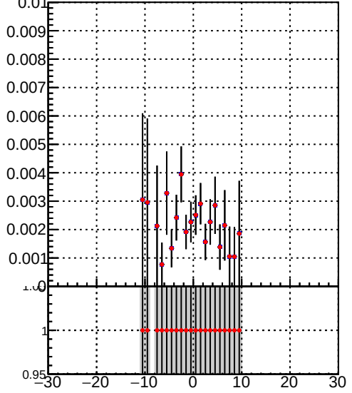
Efficiency vs sim PV z Legend: DQM_TT_mkFit-DQM_pless_orig (blue line) DQM_TT_mkFit-DQM_pless_modi2 (red line)
