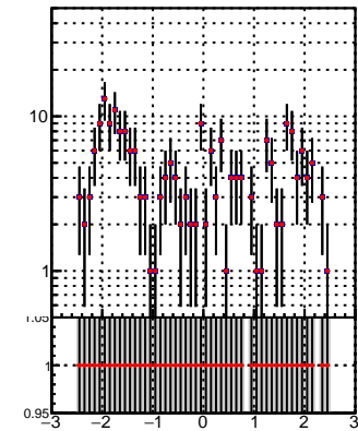
N of reco track vs \eta vs \eta —•— DQM TT mkFit-DQM pless_orig —•— DQM TT mkFit-DQM pless_modi2
