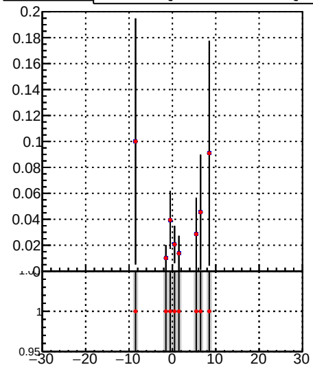
Fake rate vs vertpos Legend: DQM_TT_mkFit-DQM_pless_orig (grey line with blue dots) DQM_TT_mkFit-DQM_pless_modi2 (red line with red dots)
