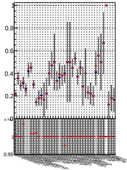
Fake rate vs. DQM_TT_mkFit-DQM_pless_orig DQM_TT_mkFit-DQM_pless_modi2
