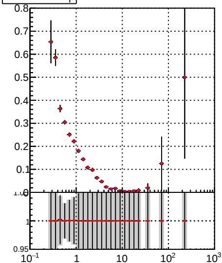
—•— DQM_TT_mkFit-DQM_pless_orig —•— DQM_TT_mkFit-DQM_pless_modi2
