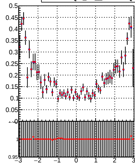
—•— DQM_TT_mkFit-DQM_pless_orig —•— DQM_TT_mkFit-DQM_pless_modi2
