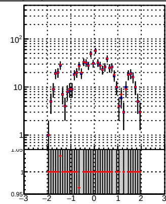
N of reco track vs \eta DQM_TT_mkFit-DQM_pless_orig DQM_TT_mkFit-DQM_pless_modi2
