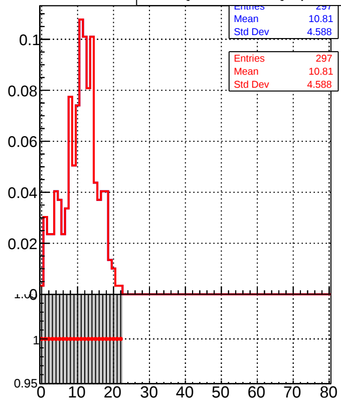
Legend for the bottom row of plots: DQM_TT_mkFit-DQM_pless_orig (Gray shaded area) DQM_TT_mkFit-DQM_pless_modi2 (Red line with markers)
