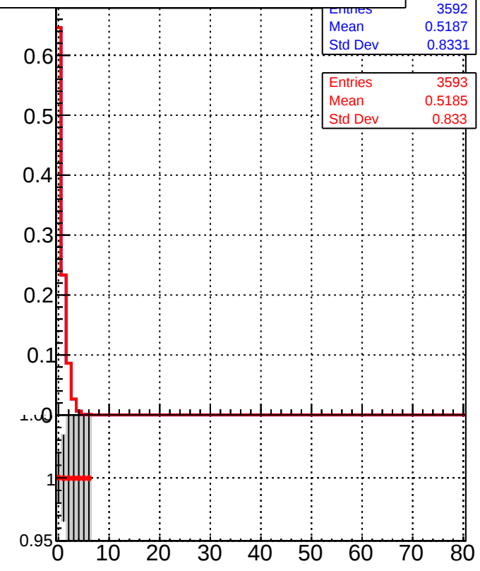
DQM_TT_mkFit-DQM_pless_orig DQM_TT_mkFit-DQM_pless_modi2
