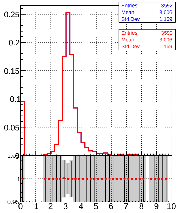
DQM_TT_mkFit-DQM_pless_orig DQM_TT_mkFit-DQM_pless_modi2
