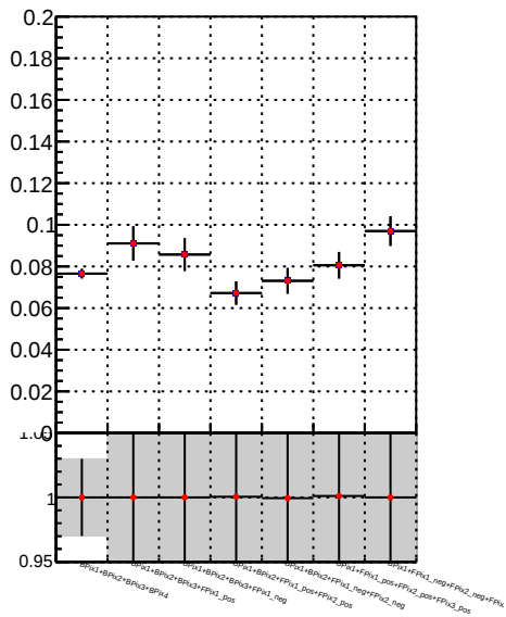
Fake rate vs. DQM_TT_mkFit-DQM_pless_orig DQM_TT_mkFit-DQM_pless_modi2
