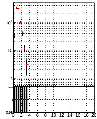
N of reco track vs. \chi^2 — DQM TT mkFit-DQM_pless_orig — DQM TT mkFit-DQM_pless_mod12
