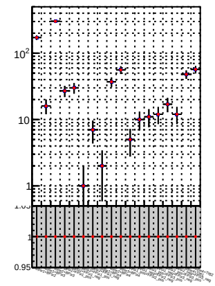
N of reco track vs. \chi^2 — DQM TT mkFit-DQM_pless_orig — DQM TT mkFit-DQM_pless_mod12
