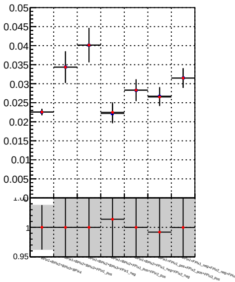
Fake rate vs. \text{DQM\_TT\_mkFit-DQM\_pless\_orig} \text{DQM\_TT\_mkFit-DQM\_pless\_modi2}
