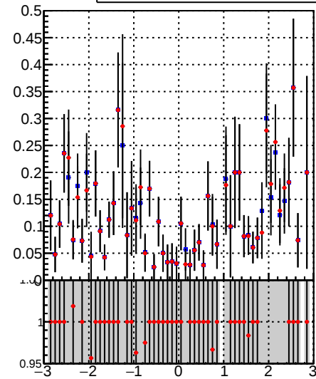
—■— DQM_TT_mkFit-DQM_pless_orig —●— DQM_TT_mkFit-DQM_pless_modi2
