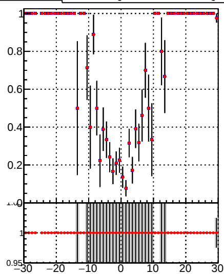
—•— DQM_TT_mkFit-DQM_pless_orig —•— DQM_TT_mkFit-DQM_pless_modi2
