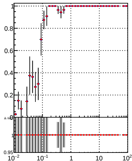
—•— DQM_TT_mkFit-DQM_pless_orig —•— DQM_TT_mkFit-DQM_pless_modi2
