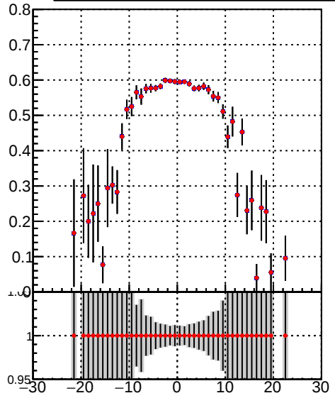
Efficiency vs vertpos Legend: DQM_TT_mkFit-DQM_pless_orig (Blue line with error bars) DQM_TT_mkFit-DQM_pless_modi2 (Red line with error bars)
