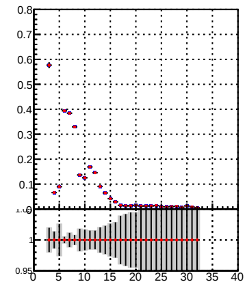
Legend: DQM_TT_mkFit-DQM_pless_orig (grey histogram), DQM_TT_mkFit-DQM_pless_modi2 (red line with error bars)
