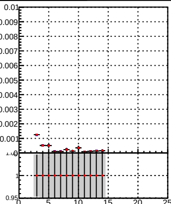
DQM_TT_mkFit-DQM_pless_orig
