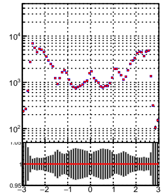
N of reco track vs \eta pT eta Legend: —•— DQM_TT_mkFit-DQM_pless_orig —•— DQM_TT_mkFit-DQM_pless_modi2
