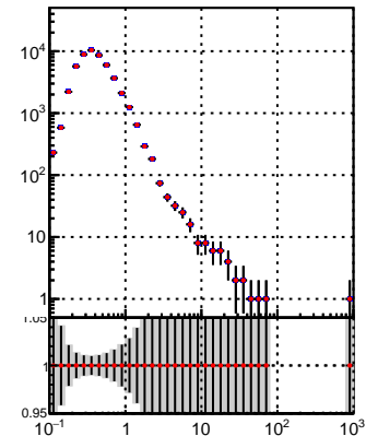
N of reco track vs \eta pT eta Legend: —•— DQM_TT_mkFit-DQM_pless_orig —•— DQM_TT_mkFit-DQM_pless_modi2
