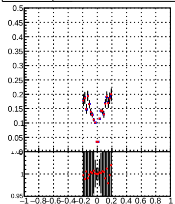
—●— DQM_TT_mkFit-DQM_pless_orig —●— DQM_TT_mkFit-DQM_pless_modi2
