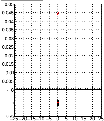
—●— DQM_TT_mkFit-DQM_pless_orig —●— DQM_TT_mkFit-DQM_pless_modi2
