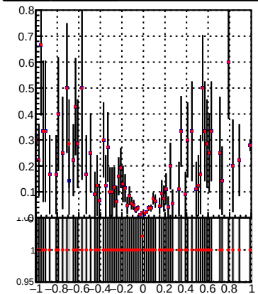
Efficiency vs Dxy(PV) Legend: DQM_TT_mkFit-DQM_pless_orig DQM_TT_mkFit-DQM_pless_mod2
