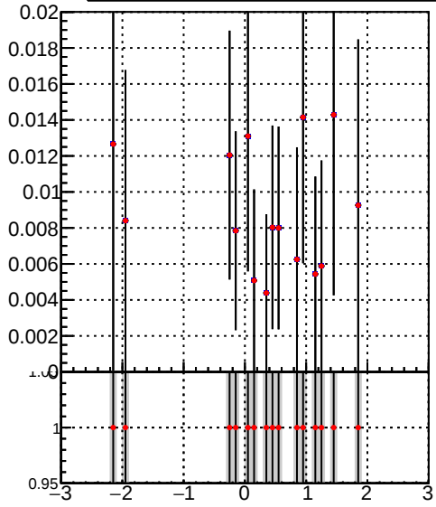
DQM_TT_mkFit-DQM_pless_orig DQM_TT_mkFit-DQM_pless_modi2
