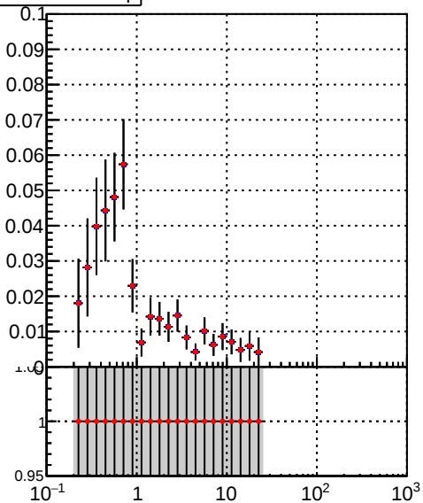
■ DQM_TT_mkFit-DQM_pless_orig ● DQM_TT_mkFit-DQM_pless_modi2
